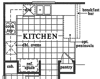
OPT. COOKTOP WITH DOUBLE OVENS AT KITCHEN
