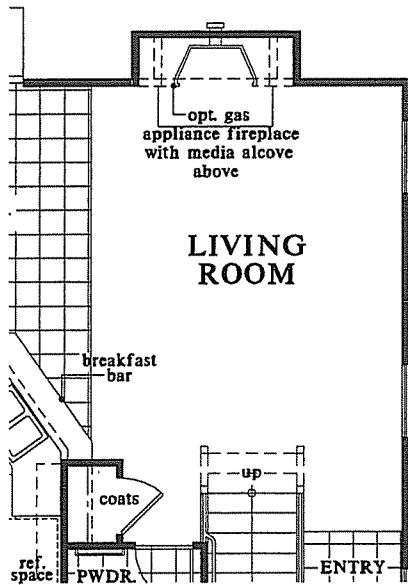
OPT. GAS APPLIANCE FIREPLACE WITH MEDIA ALCOVE AT LIVING ROOM
