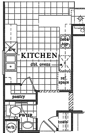
OPT. COOKTOP WITH DOUBLE OVENS AT KITCHEN
