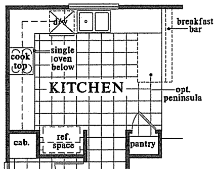
OPT. COOKTOP WITH SINGLE OVEN BELOW AT KITCHEN
