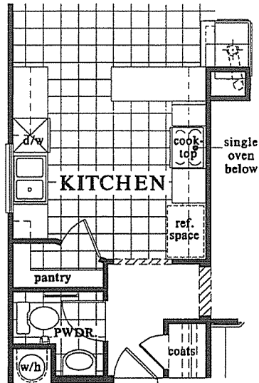
OPT. COOKTOP WITH SINGLE OVEN BELOW AT KITCHEN
