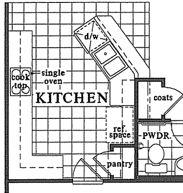
OPT. SEPARATE COOKTOP OVER SINGLE OVEN AT KITCHEN
