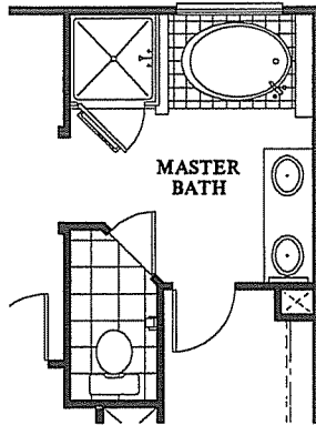
OPT. ACRYLIC OVAL TUB WITH SEPARATE SHOWER AT MASTER BATH
